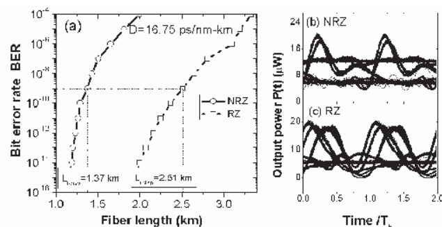
Fig. 3 BER versus fiber length L_f with fiber dispersion, (a), and the simulated eye diagrams under (b) NRZ modulation and (c) RZ modulation. The maximum fiber length L_{f-disp} corresponds to BER = 10^{-9}
