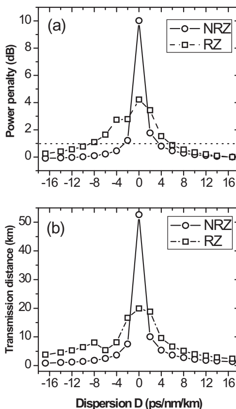
Fig. 6 Influence of varying the fiber dispersion by using NZ-DSF on (a) the power penalty of the 40-Gbps fiber system and (b) the dispersion-limited fiber length L_{f-disp} under NRZ and RZ modulation bit patterns
