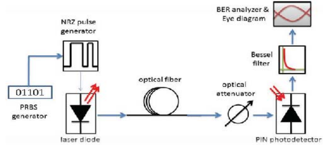
Fig. 1 Scheme of the designed fiber communication system
