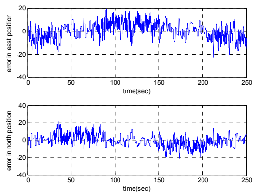
Fig. 20 Position error between the true and simulated GPS trajectories
