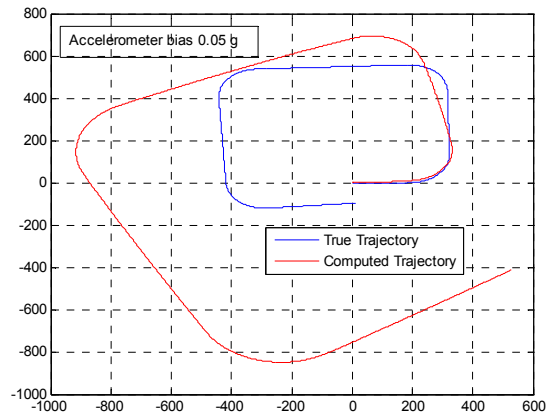
Fig. 13 Reference and INS derived trajectories with 0.05g accelerometer bias
