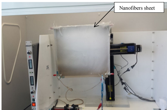
Fig. 1 Electrospinning setup
