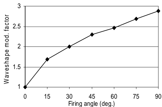
Fig. 6 Variation of wave shape modification factor ( K_S )
