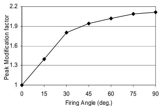
Fig. 5 Variation of peak modification factor ( K_P )
