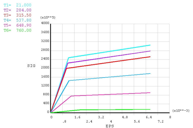
Fig. 2 Elasto-plastic stress-strain
