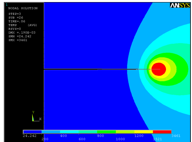
Fig. 6 Temperature contour
