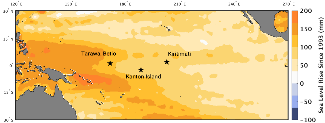
Figure ES 1: Amount of sea level rise (mm) from 1993 to 2022 estimated from satellite altimetry data. Stars indicate the locations of the tide gauges in the Gilbert (Tarawa), Phoenix (Kanton Island) and Line (Kiritimati) Islands.
