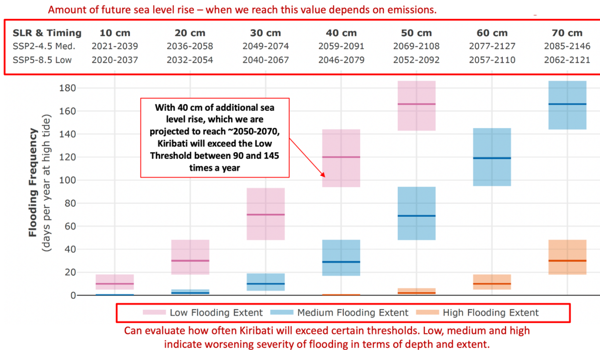
Figure A1. Annotated example of flood frequency figure. Shown here is the figure for Tarawa, corresponding to Figure 8 in the report above. The red text box on the graph itself provides an example of the type of statement that can be generated using this analysis.
