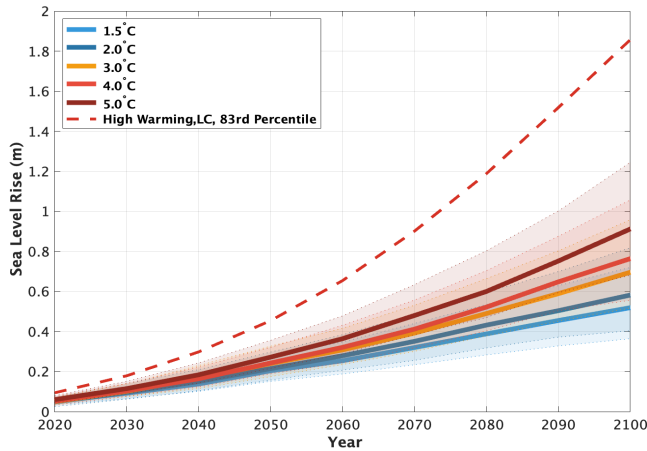
Figure ES 3: Projections of future sea level rise from 2020 to 2100 for Kiribati in meters, relative to 2005. Shaded regions represent the likely range for each projection, and the red dashed line represents a plausible upper limit.
