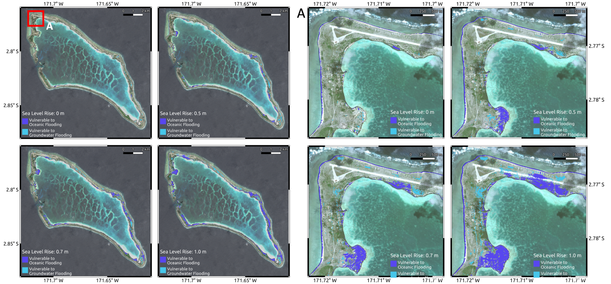
Figure 9. Projected inundation for 0 cm, 50 cm (Low), 70 cm (Medium) and 100 cm (High) of sea level rise over current MHHW for Kanton Island, with an inset of the airport (A). Light blue denotes areas below future MHHW, but not necessarily connected to the sea, while dark blue areas are projected to be directly inundated from the sea. Note, this assumes no additional protection or adaptation beyond what is currently implemented.
