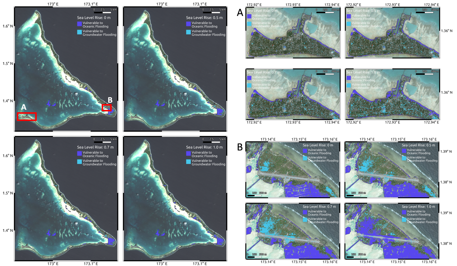
Figure 7. Projected inundation for 0 cm, 50 cm (Low), 70 cm (Medium) and 100 cm (High) of sea level rise over current MHHW for Tarawa, with insets of the port (A) and airport (B). Light blue denotes areas below future MHHW, but not necessarily connected to the sea, while dark blue areas are projected to be directly inundated from the sea. Note, this assumes no additional protection or adaptation beyond what is currently implemented.
