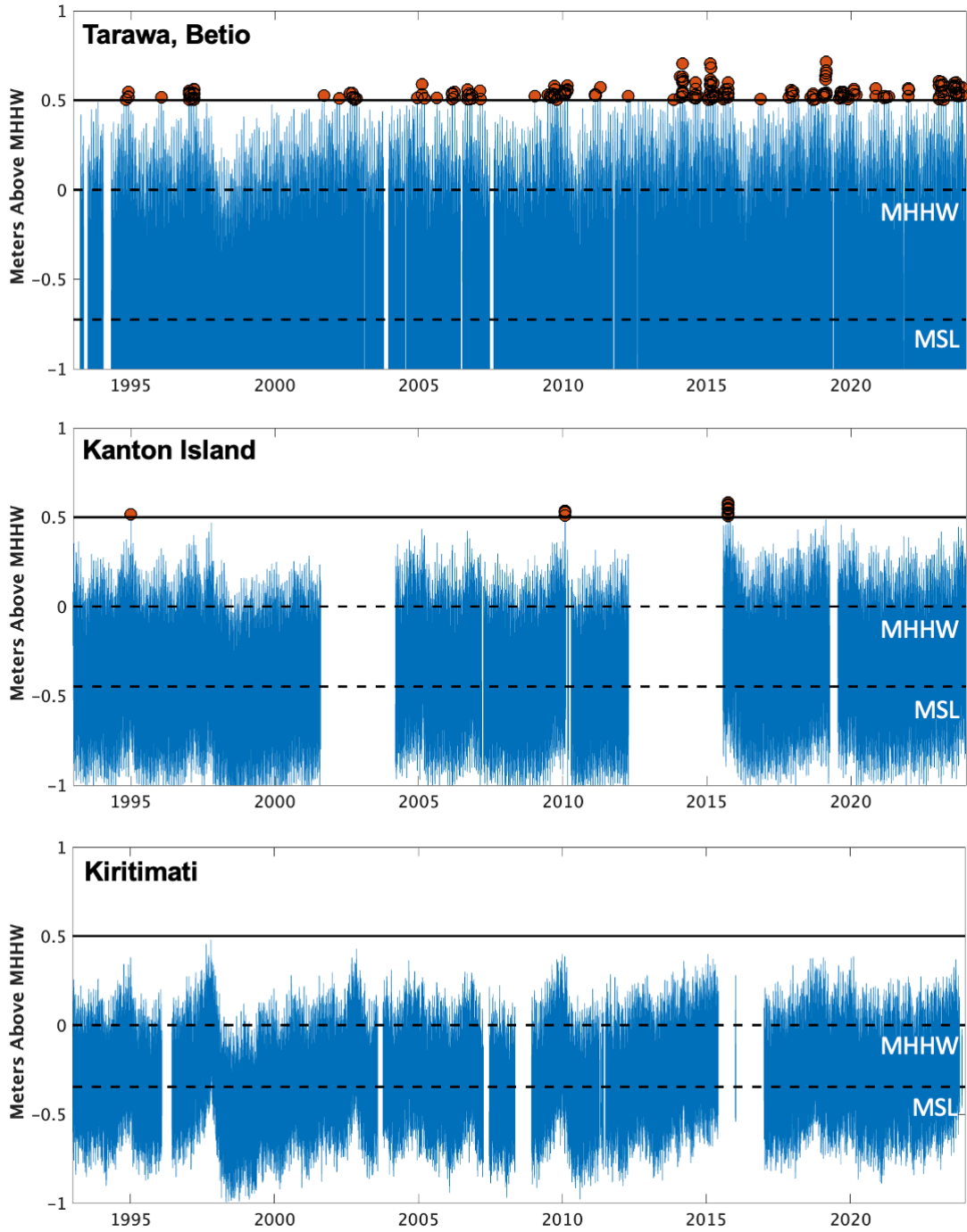
Figure 3. The range of hourly total water levels (blue) for the tide gauge records in Kiribati are shown with mean sea level (MSL; dashed black line), mean higher high water (MHHW; dashed black line), and a 50 cm above MHHW flooding threshold (solid black line). The occurrence of individual flooding days above this threshold (red circles) are not distributed evenly throughout the year and tend to occur in January, February and March, coinciding with the highest tides of the year. (Adapted from source: https://pacificislandsflooding.org/projected-flooding ).
