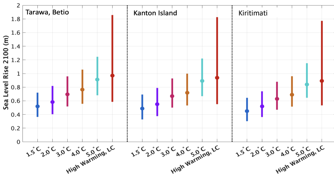
Figure 4. IPCC AR6 Projections in 2100 for three locations across Kiribati showing levels of sea level rise relative to 2005. Projections are shown for each AR6 scenario. Circle markers indicate the median projection, while the bars represent the 17 th -83 rd percentile confidence interval.
