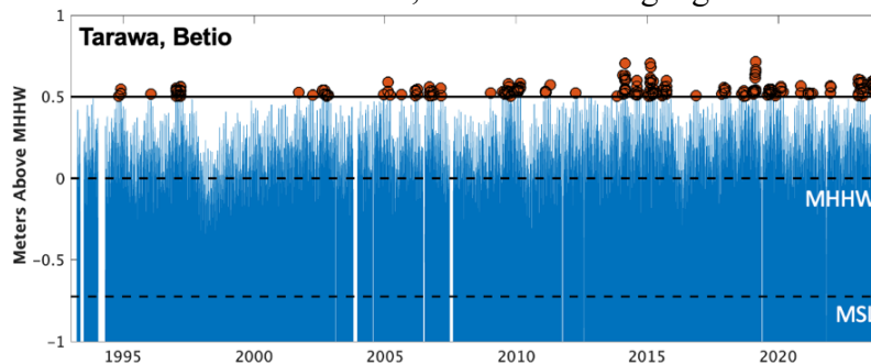
Figure ES 2: The range of total water levels (blue) for the tide gauge records in Tarawa, with flooding days (red circles), where the water level exceeded 50 cm above mean higher high water (MHHW). Mean sea level (MSL) is also shown.
