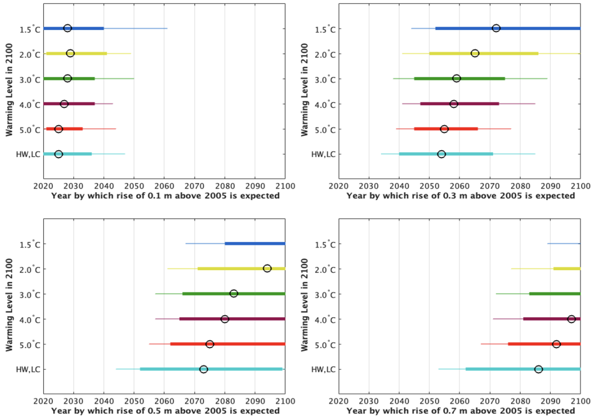
Figure 6. Timing of exceedance of different thresholds of 0.1 m (top left), 0.3 m (top right), 0.5 m (bottom left) and 0.7 m (bottom right) under different warming level projections. Thick bars show 17th-83rd percentile ranges, and black circles show median values. Thin bars show 5th-95th percentile ranges.
