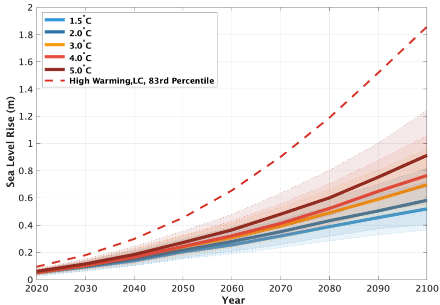
Figure 5. Projections of future sea level rise from 2020 to 2100 for Kiribati in meters, relative to 2005. The shaded regions represent the likely range for each projection, and the red dashed line represents a plausible upper end estimate for sea level rise.
