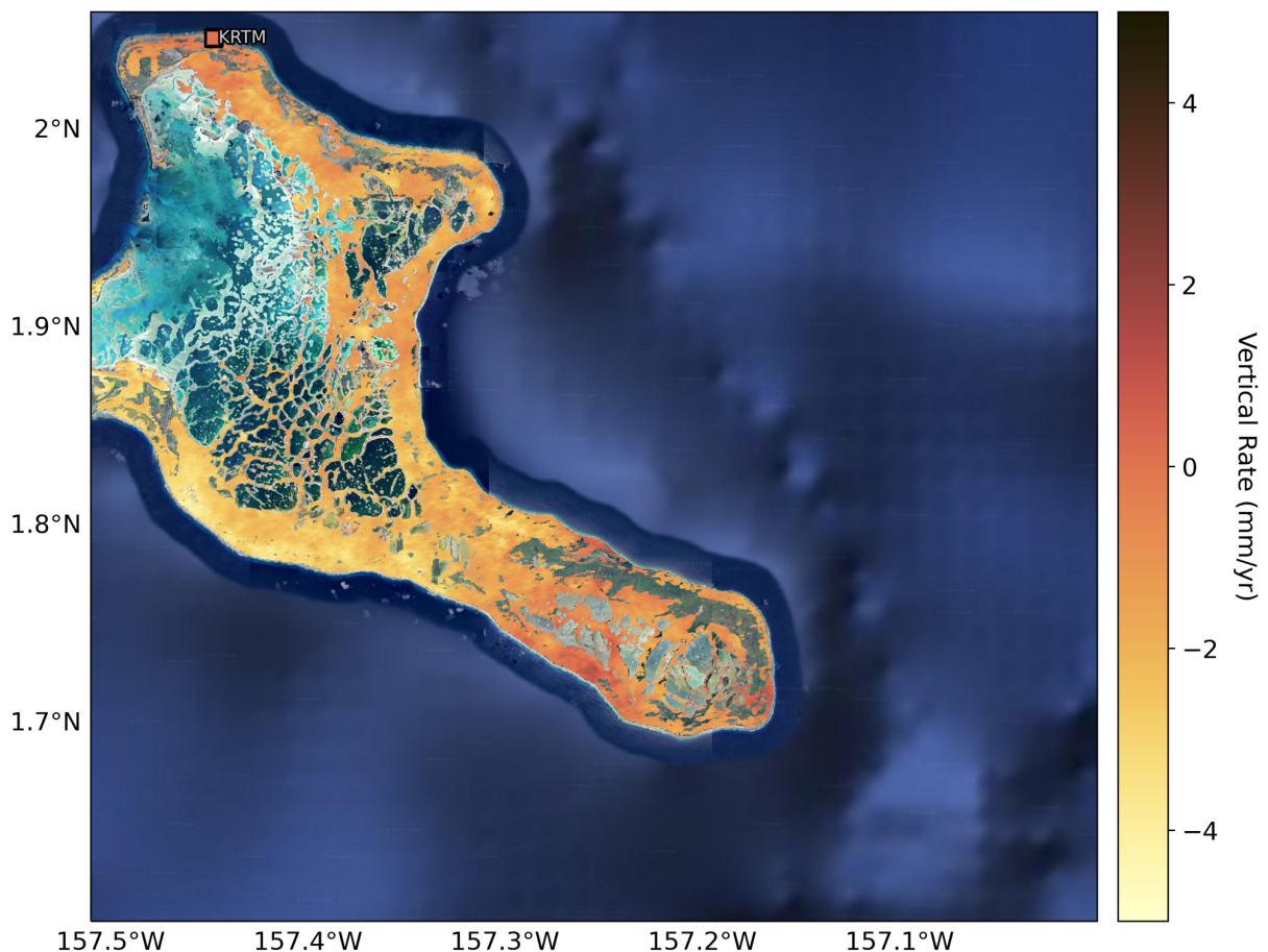
Figure 13. InSAR-estimated map of vertical land motion for Kiritimati from Sentinel-1 satellite observations over the period from 2014 to 2023. The map indicates broadscale subsidence with some spatial variability in the rate of subsidence across the island.
