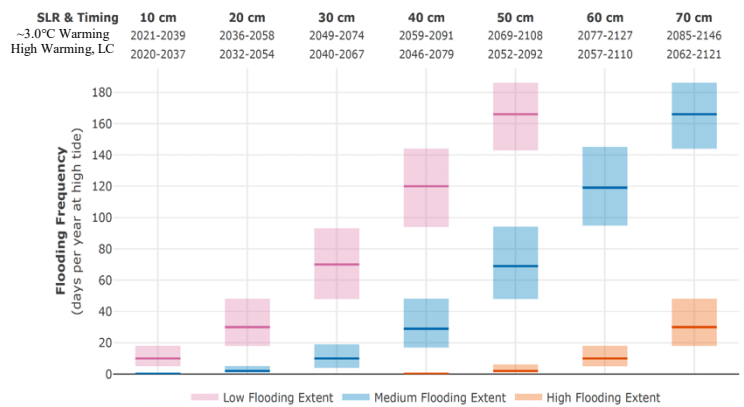
Figure ES 4: Flooding frequency in Tarawa for different amounts of future sea level rise (10-70 cm) above current MHHW, shown with timings for the ~3.0°C warming, medium confidence scenario and the high warming, low confidence scenario.
