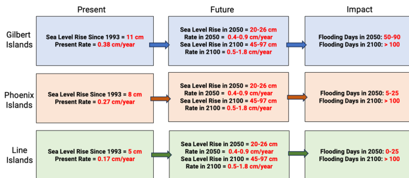
Figure ES 3: Summary of current sea level rise and future projections for rates of sea level rise and flooding occurrence
