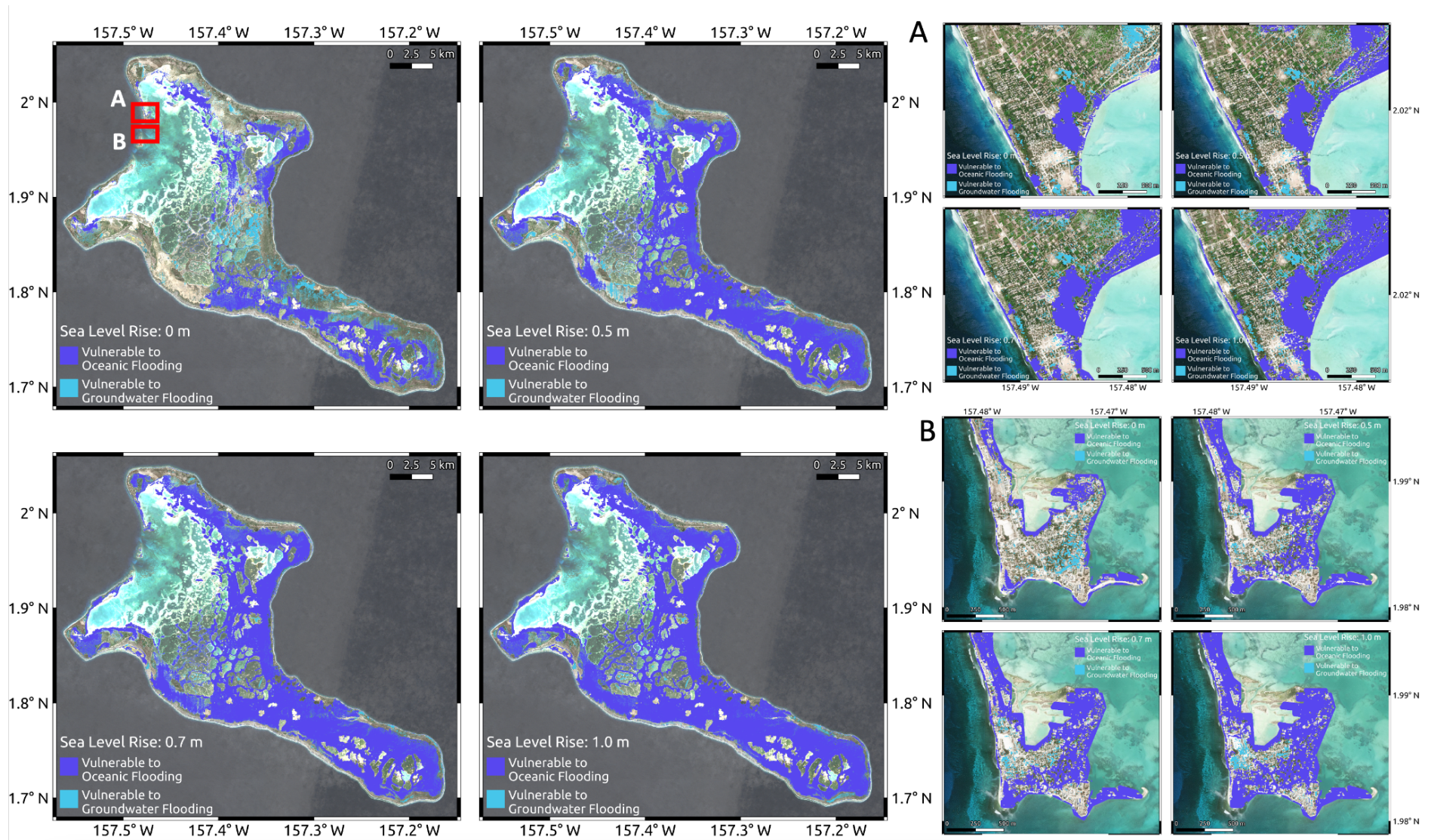
Figure 11. Projected inundation for 0 cm, 50 cm (Low), 70 cm (Medium) and 100 cm (High) of sea level rise over current MHHW for Kiritimati. Light blue denotes areas below future MHHW, but not necessarily connected to the sea, while dark blue areas are projected to be directly inundated from the sea. Note, this assumes no additional protection or adaptation beyond what is currently implemented.
