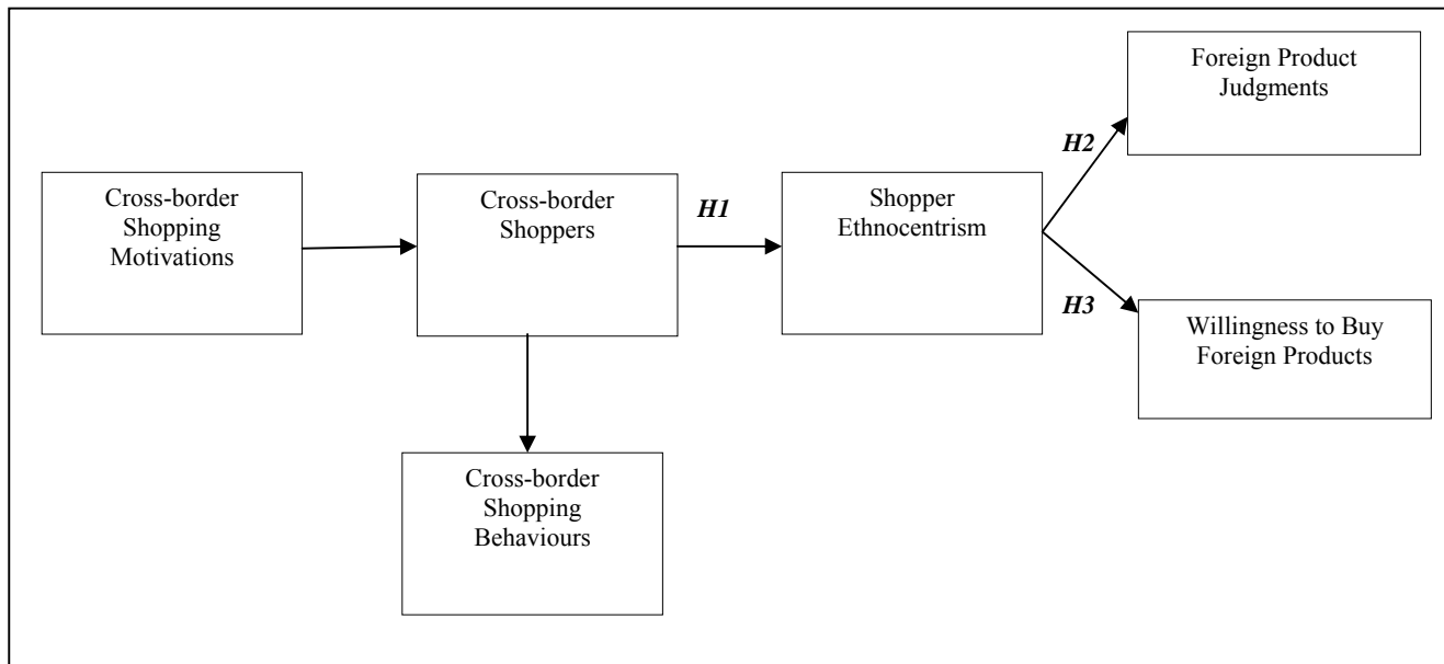
Fig. 1 Conceptual Model
