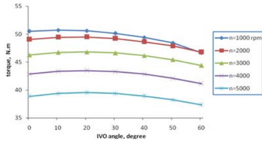
Fig. 2 Torque versus IVO degree for different speeds
