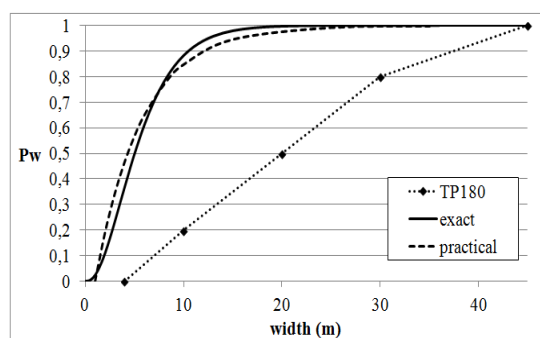
Fig. 2 Category roe deer – dependence of P_w on width of the underpass (m)
