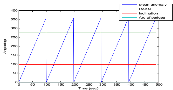
Fig. 5 Keplerian Elements from MATLAB
