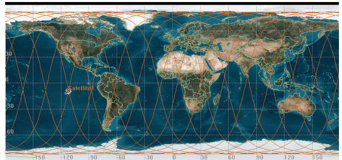
Fig. 3 Ground Track of ICUBE-1
