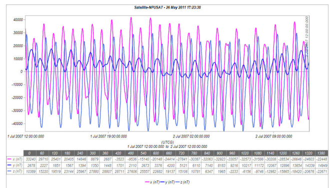
Fig. 15 Geomagnetic Field Estimation in ECEF from STK
