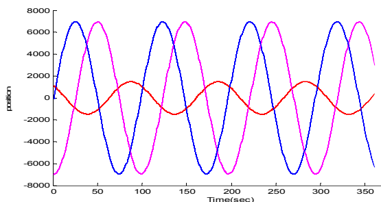
Fig. 7 Position Vector in ECI Frame from J2 Orbit Propagator
