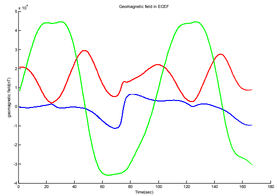
Fig. 14 Geomagnetic Field Estimation in ECEF
