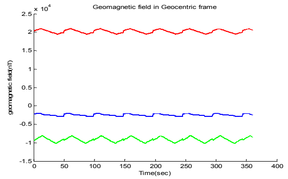
Fig. 13 Geomagnetic Field Estimation in Geocentric Frame
