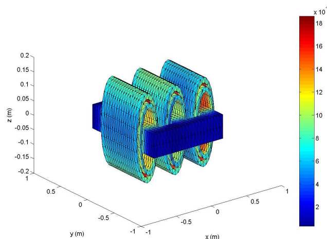
Fig. 5 Magnetic vector potential distribution (wb//m) of the transformer coil for phase unbalance case
