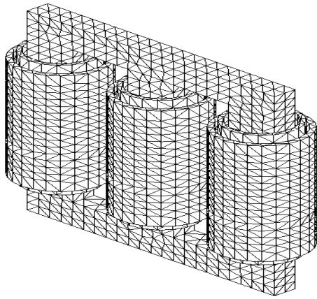
Fig. 2 Discretization of the system given in Fig. 1
