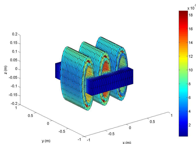
Fig. 4 Magnetic vector potential distribution (wb//m) of the transformer coil for magnitude unbalance case
