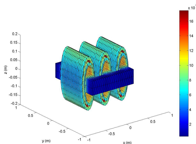
Fig. 3 Magnetic vector potential distribution (wb//m) of the transformer coil for load balancing case
