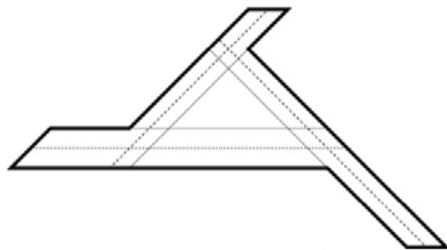
Fig. 4 A non-star-shaped polygon with chords in the three directions from which the polygon is weakly visible
