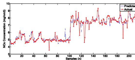
Fig. 4 NO x testing data for BPNN
