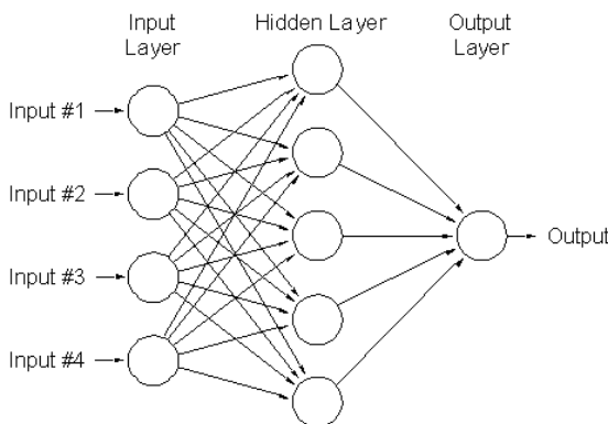
Fig. 1: Typical Backpropagation Neural Network
