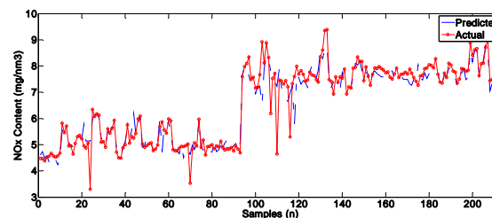
Fig. 6 NO x testing data for LS-SVR
