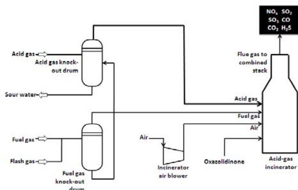
Fig. 2 PFS of incinerator train
