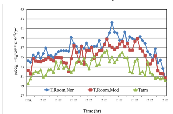
(a) Hourly variation of Room temperature
