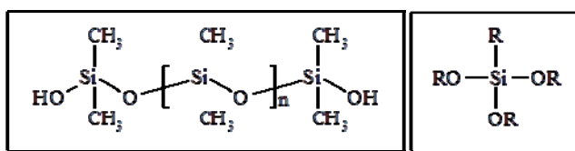
Fig. 1 Polydimethylsiloxane and alkyltrialkoxysilane
