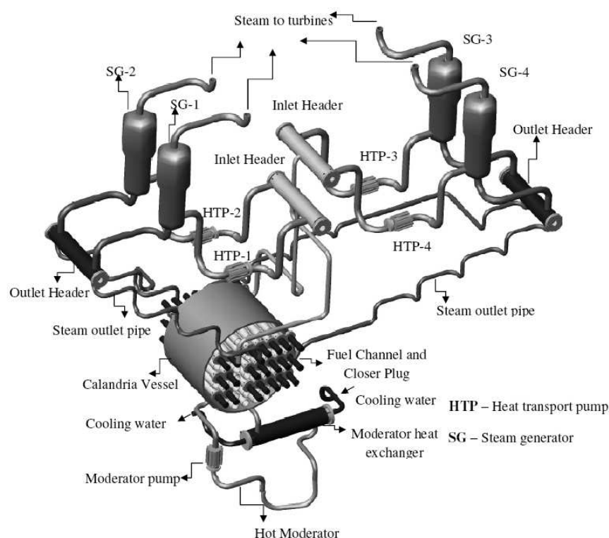
Fig. 1 Schematic diagram of heat transportation system
