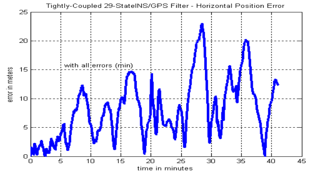
Fig. 28 The horizontal position error (TC)
