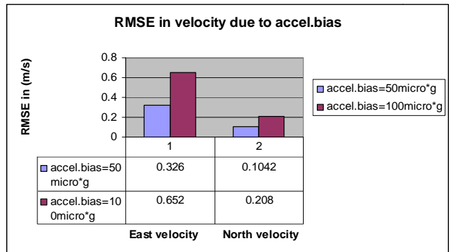
Fig. 10 RMSE in velocity due to accelerometer bias
