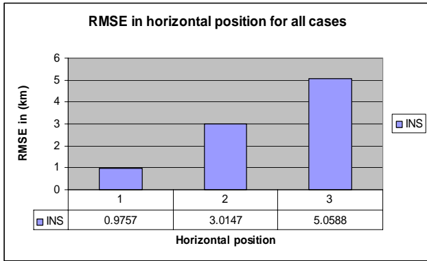
Fig .17 RMSE in horizontal position for all cases
