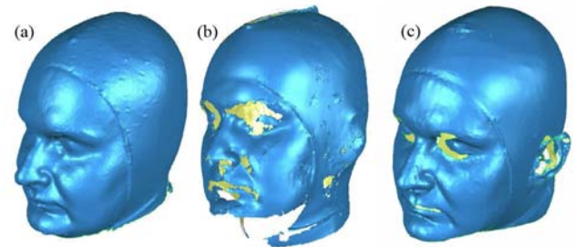
Fig. 7 Head scanning results (a) Artec MH, (b) ATOS I, (c) zSnapper
