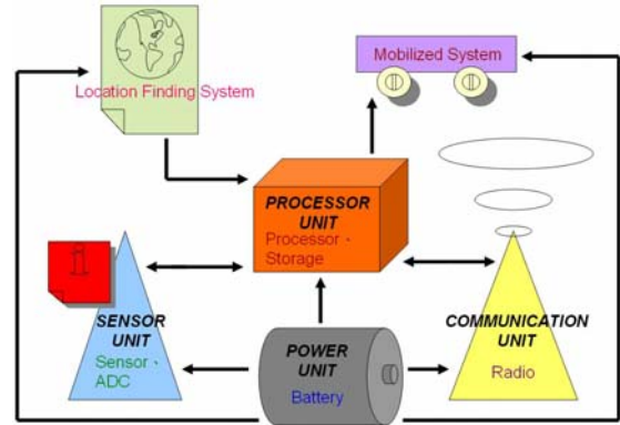
Fig 2. The basic units of a sensor device
