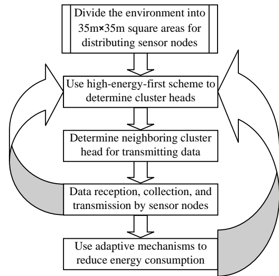
Fig. 4 The flowchart of dynamic routing method
