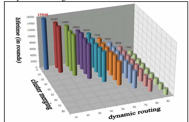
Fig. 13 Lifetime vs. timing (thresholds of electric power) for applying adaptive mechanisms with dynamic routing first
