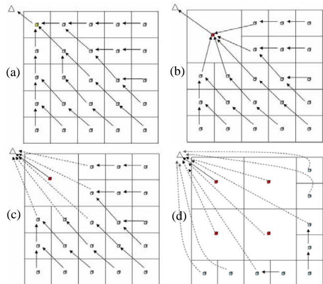
Fig. 7 The operation of cluster merging mechanism
