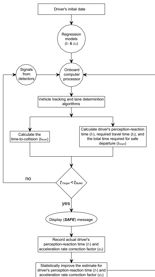
Fig. 2 Flow chart for the proposed algorithm
