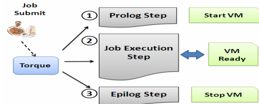
Fig. 2 VM life cycle in batch system
