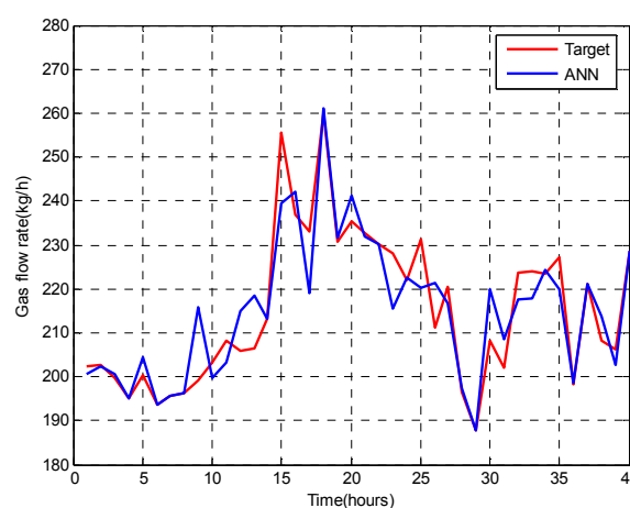
Fig. 6 Comparison of gas flow rate with testing data set 1 and 5-1 network
