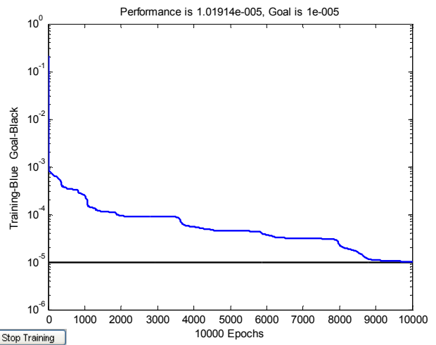
Fig. 17 Gas flow rate error with training data set 2 and 10-1 network
