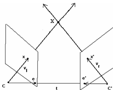
Fig. 4 Triangulation method. Due the fact the correspondent pixels (\mathbf{x}, \mathbf{x}') satisfy the epipolar constraint, the rays of \mathbf{x} and \mathbf{x}' intersect in space point \mathbf{X} .
