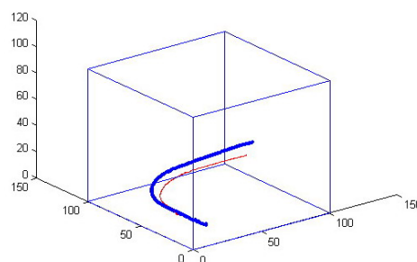
Fig. 5 Training 3D edge (red) and edge extracted in the execution step (blue)
