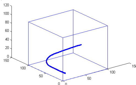
Fig. 6 The registration algorithm result. The training edge overlaps the edge extracted in the execution step
