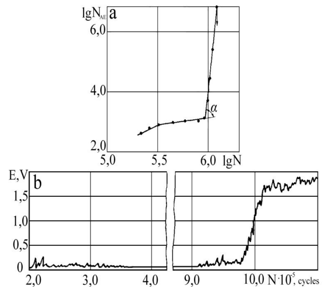
Fig. 5 The change of total (a) and energy (b) of AE signals in the process of cyclic loading of a cooled working blade (the point at which the tests were stopped is shown with an arrow)
