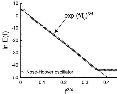
FIG. 3: Power spectrum for the Nose-Hoover oscillator. The data for the computations were taken from Ref. [18]).
