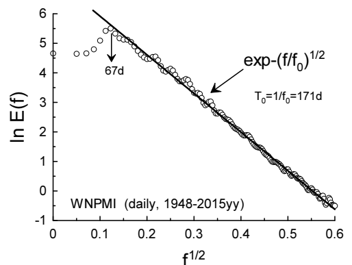
FIG. 14: Power spectrum for the intraseasonal daily WNPM index for the period 1948-2015yy (the data for the computation were taken from the site [41]).
