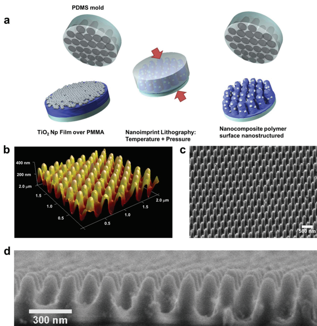
Fig. 1 (a) Scheme of the fabrication process of AR moth-eye nanocones on PMMA– \text{TiO}_2 nanocomposites. (b–d) Morphological characterization of a P-05T-AR substrate surface, (b) 3D-AFM topography image, (c) SEM image of a tilted sample, (d) SEM image of the cross-section.
