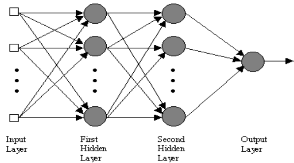
Fig. 5 Network architecture
