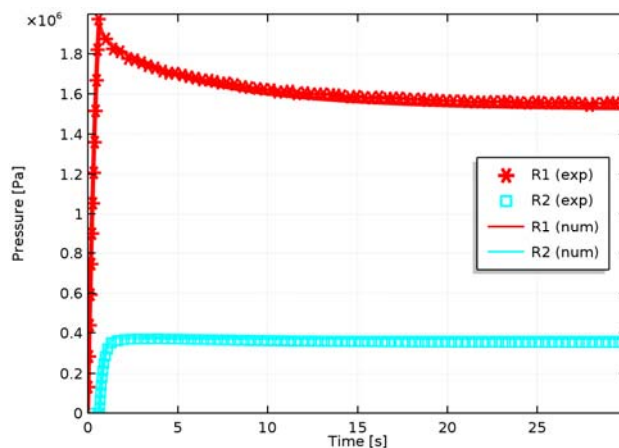
Fig. 4 Pressure difference comparison in ( R_1 ) between experimental and simulated data: return to equilibrium
