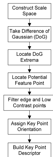
Fig. 3 SIFT Algorithm
