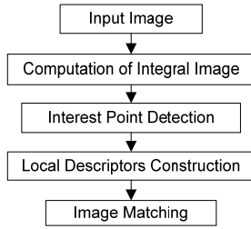
Fig. 4 SURF Algorithm
