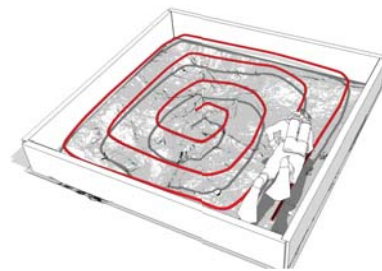
(b) The spiral method was the ideal survey trajectory in < 0.5m visibility conditions as it kept more than 50% overlap between the images
