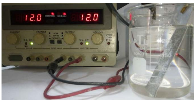
Fig. 3 Anodizing of Aluminium in 12 wt.% Phosphoric acid at 12V
