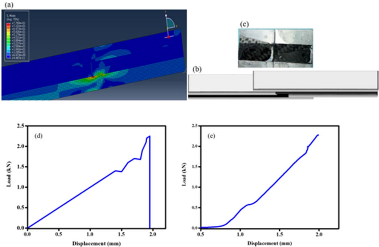
Fig. 6 (a) Simulated stepped lap joint, (b) Stepped lap joint design (c) Sample after testing showing cohesive failure. Load vs displacement curve of (d) simulated (e) experimented
