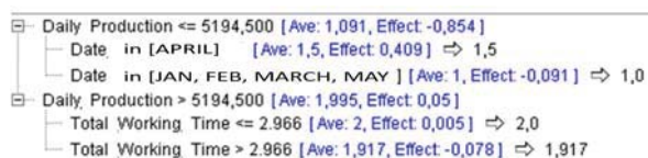
Fig. 3 CART model results for production per person
