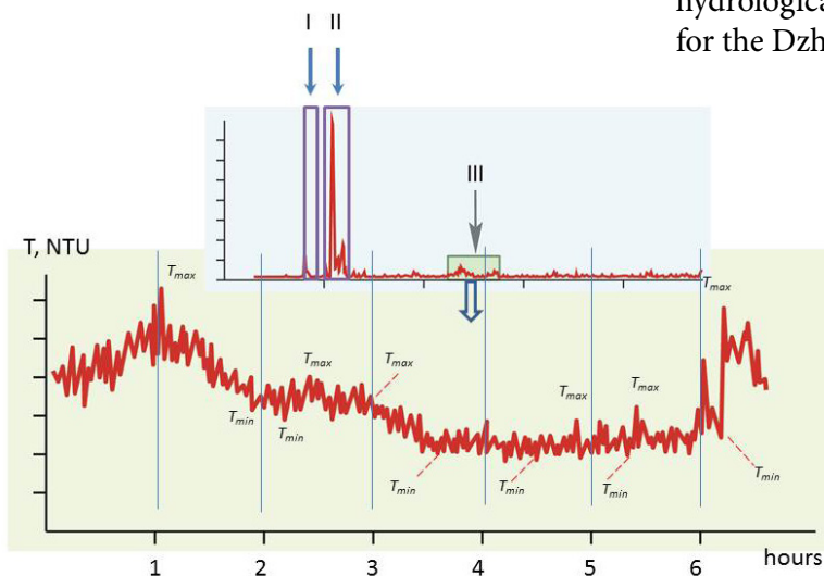
Figure 2. Method of sedigraph separation (I, II, III – hydrological events (HE)). An example of the breakdown into hydrological events and the calculation of the TI index for the Dzhankuat river (8 th station).
