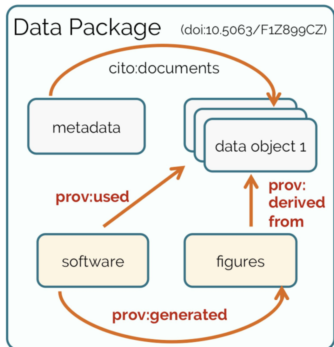
Figure 1: A DataONE Data Package is a composite container for data, software, and visualizations, and the metadata that describes these. Provenance relationships link the objects within and across packages into computational workflows for reproducible science.
