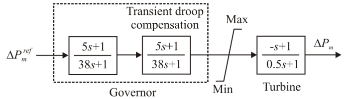
Fig. 1. Block diagram of hydraulic unit [20].
