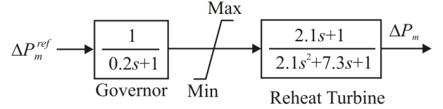
Fig. 2. Block diagram of reheat unit [20].
