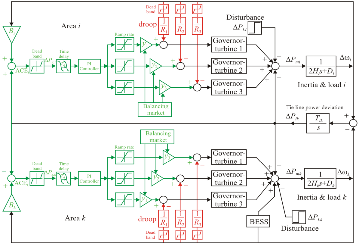
Fig. 5. Power system model used for the study.
