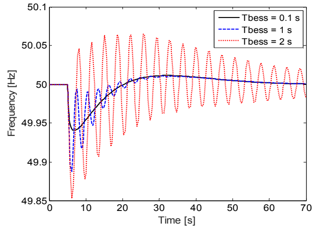
Fig. 10. Influence of the BESS time response on the frequency stability.
