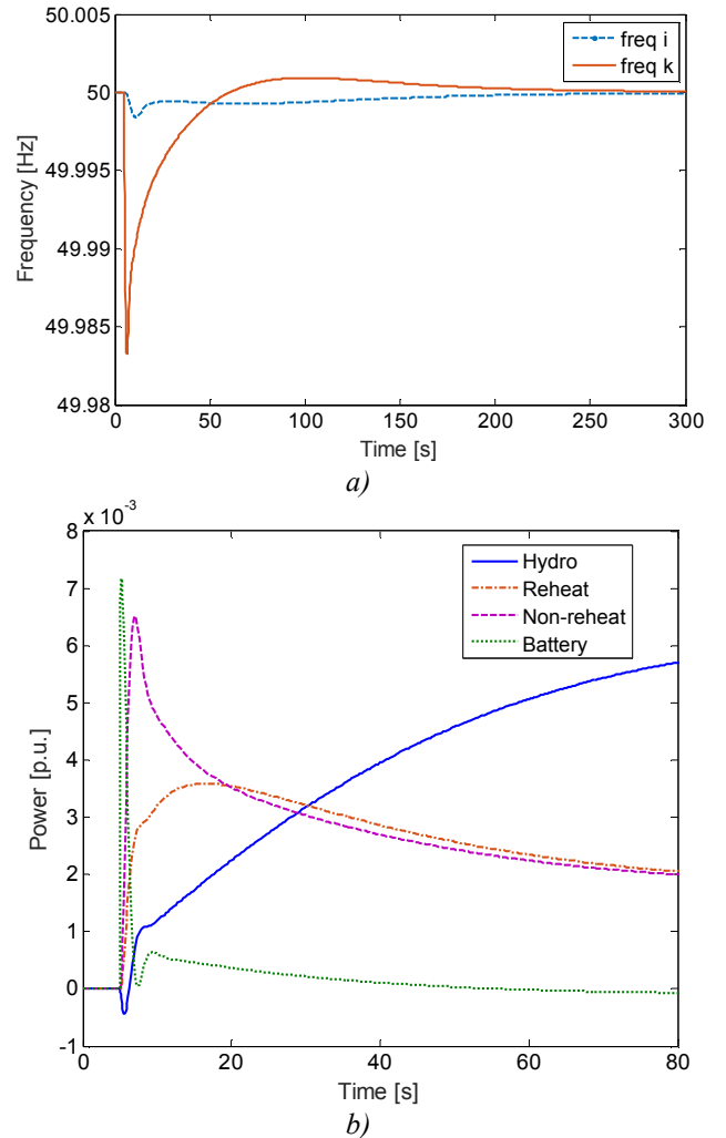
Fig. 7. System behaviour under normal inertia value and all types of generation units considered for frequency control.
