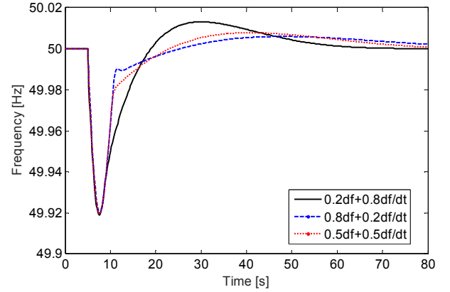
Fig. 9. Frequency response for battery having reserve limits.
