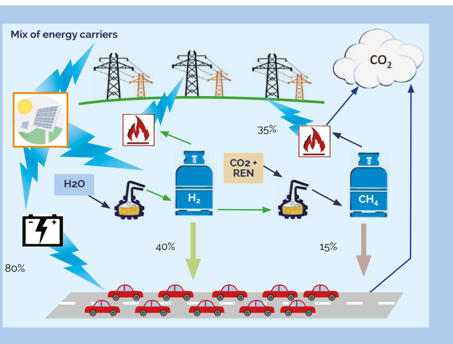
Figure 5.4: A combined technology system.
