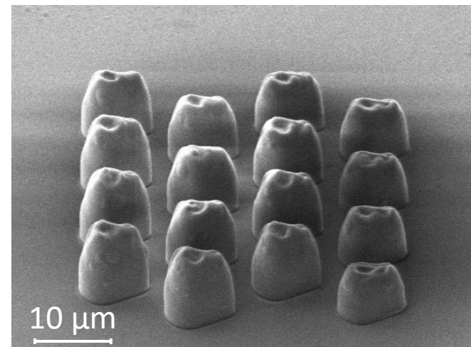
SEM images of Two Photon Polymerization structures
