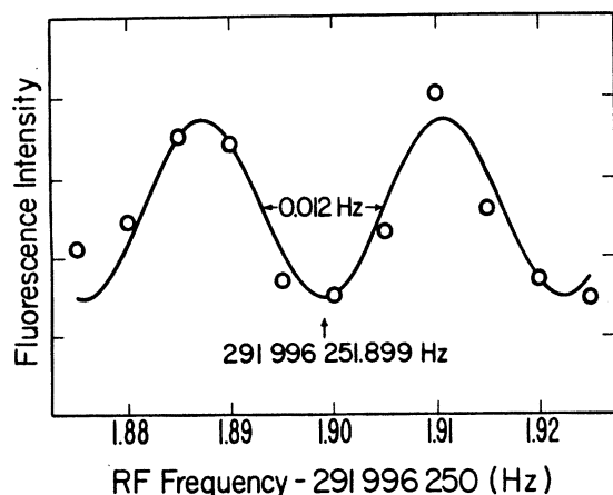
Figure 3. ^{25}\text{Mg}^+ hyperfine resonance.
