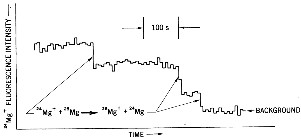
Figure 2. Fluorescence from a small cloud of ^{24}\text{Mg}^{+} ions. The three large steps are due to the loss of individual ions.
