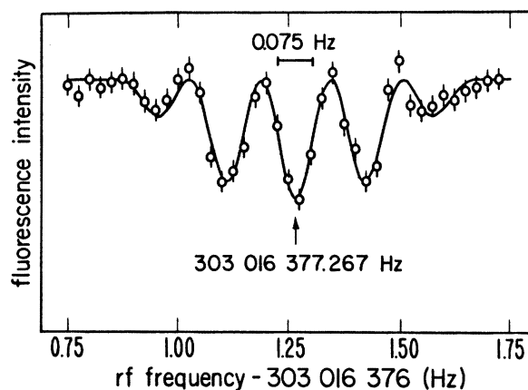
Figure 4. ^9\text{Be}^+ hyperfine resonance.
