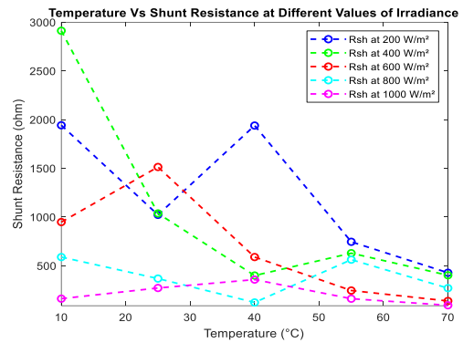
Figure 8 Temperature vs. Shunt Resistance at Different G
