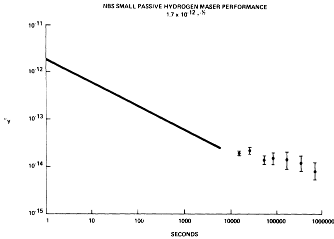
Fig. 5. Frequency stability of small hydrogen maser based on 32-day comparison simultaneously against 8s and a cesium standard NBS-4.
