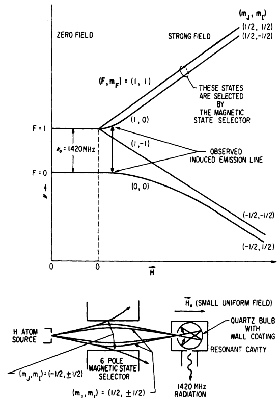
Fig. 1. Magnetic hyperfine transition of hydrogen atom (above). Hydrogen maser schematic (below).
