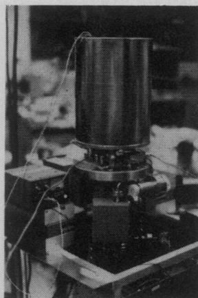
Fig. 4. Completed prototype cavity assembly with four nested magnetic shields.
