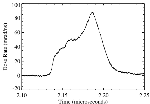
Figure 7. Plot of the x-ray dose rate for a show with 20% higher Marx charge voltage.
