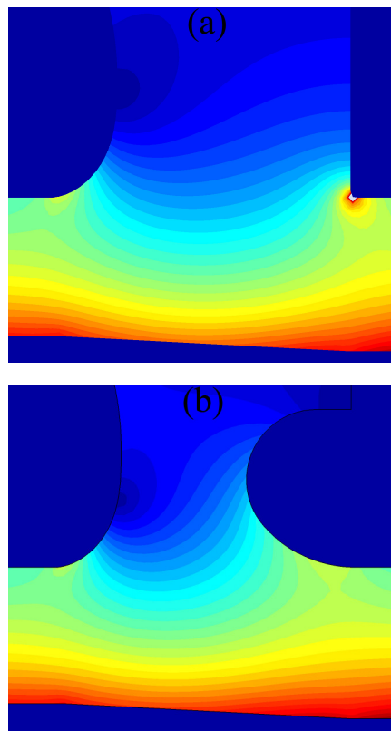
Figure 2. Electrostatic field plots of the electric field magnitude at the output of the last IVA cell. (a). Original design with sharp cathode edge. (b). New field shaper design.
