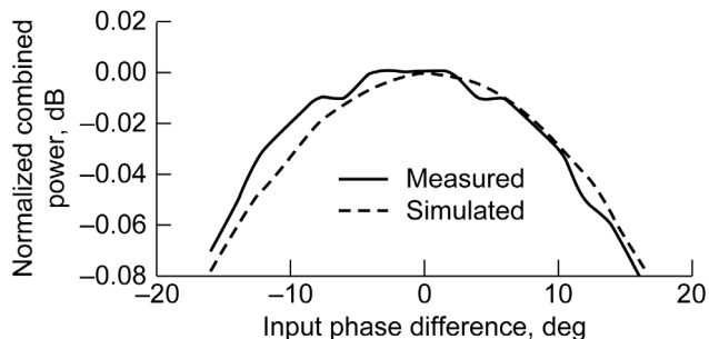
Fig. 10. Measured and simulated normalized combiner power output as a function of input phase difference.
