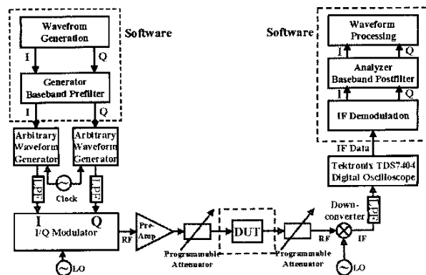
Figure 1. Schematic of the Ultra-Wideband Vector Signal System.
