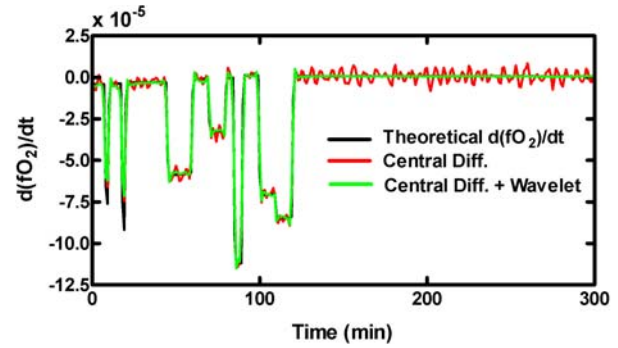
Fig. 1. The derivative of a simulated room O_2 concentration, d(f_{O_2})/dt , corrupted by colored noise. The Central Difference method of calculating the d(f_{O_2})/dt (red line) captures sharp changes, but contains significant noise during the steady-state period ( >150 min). Applying the wavelet transform to the central difference (green line) reduces the noise while retaining sharp features.
