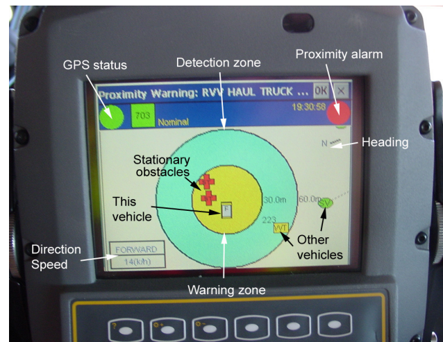
Figure 8. Driver interface for GPS-based proximity warning system.
