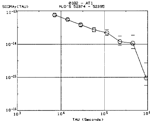
Figure 1: Sample root Allan variance \sigma_y(\tau) (referred to as Avar the best, or maximum-overlap estimator) of a commercial Cs frequency standard vs. NIST’s AT1 time scale. In the long-term \tau -region, we see variations which may be interpreted as having a quasi-sinusoidal modulation in the data at long term (note the existence of peaks and dips near the longest term values).
