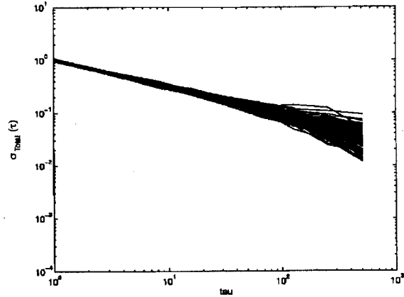
Figure 4: Not only is root Totvar less variable, but its response is smoother with fewer oscillations at long-term with the same 100 simulation trials of WHFM noise as in figure 3.
