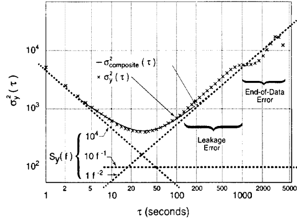
Figure 2: Note the apparent presence of quasi-sinusoidal data indicated by the oscillatory response at long-term of the sample Allan variance \sigma_y^2(\tau) due to sampling errors (the noise simulation represents the linear addition of three power-law noise types and should result in the “composite” solid curve) [6].
