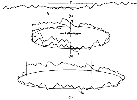
Figure 7: Circular extension of the original x(t) data set for computation of Total variance.
