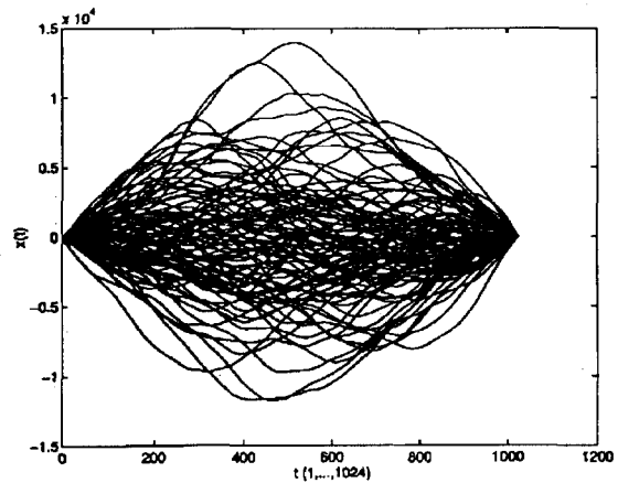
Figure 6: 100 segments of \{x_t\} as simulations of random walk FM in which a slope is removed so that the ends are matched. Note that the random shape often appears as about one-half or one sinusoidal cycle over the entire sample interval.
