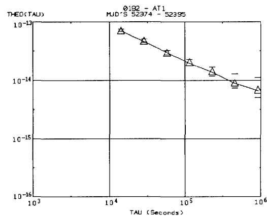
Figure 8: Long-term frequency stability can also be calculated using a new statistic called "Theo1," which shows virtually none of the oscillatory behavior inherent in the Allan deviation. Shown above is a plot of Theo1 (interpreted exactly as the usual sigma-tau, or Allan deviation, plot) that uses the same data used to compute the Allan deviation, or root Avar, in figure 1.
