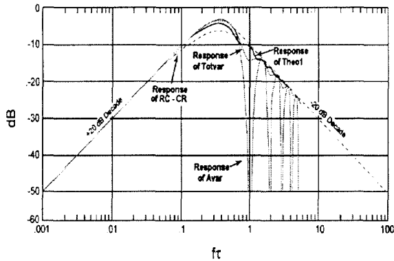
Figure 5: A comparison of frequency responses acting on y(t) of Avar, Totvar, and a passband variance considered to be ideal consisting of a simple cascade of a single-pole high-pass followed by a low-pass filter with identical break points at RC = \tau/2 (dashed curve). Totvar side lobes are flatter and closer to ideal without Avar's deep nulls at large \tau . The dark solid line is the frequency response of a new statistic called "Theol" and which exhibits the lowest passband ripple.
