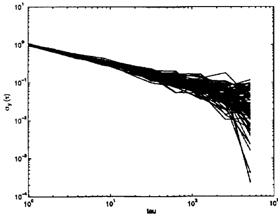
Figure 3: Oscillatory response at long term shows up frequently in the classical sample root Allan variance \sigma_y(\tau) with 100 simulation trials of WHFM noise.
