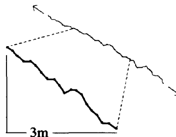
Figure 3. Procedure for TotalMod- \sigma_y(\tau) , Total- \sigma_x(\tau) , and Total- \sigma_H\sigma_y(\tau) starts with original data subsequence.
