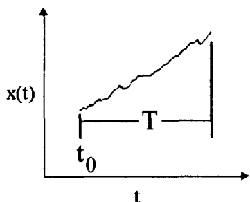
Figure 1. Original data stream, \{x_n\} .
