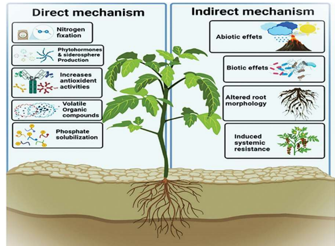
Fig. 2. Direct and indirect mechanism of PGPR.
