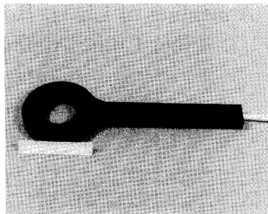
Fig. 3. A packaged coil. Coil diameter is approximately 5 cm. The package is 30 cm long.
