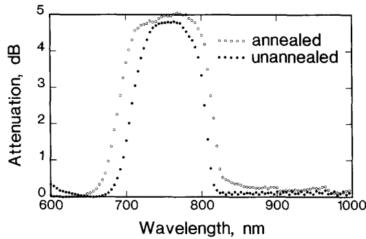
Fig. 4. Spectral attenuation of annealed and unannealed coils of a fiber with Ge:SiO 2 core and SiO 2 cladding. NA = 0.138.
