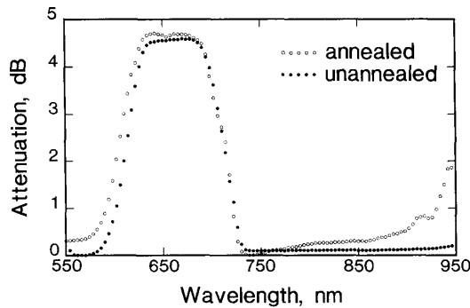
Fig. 6. Spectral attenuation of annealed and unannealed coils of a fiber with Ge:SiO 2 core, slightly depressed inner cladding doped with phosphorus and fluorine, and SiO 2 cladding. NA = 0.13.
