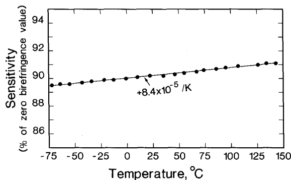
Fig. 13. Sensitivity versus temperature data for the unpackaged coil of Fig. 9.
