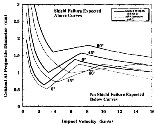
Figure 8. Ballistic Limits of Stuffed Whipple (MOD-2) and All-Aluminum (Al-2) Shields.
